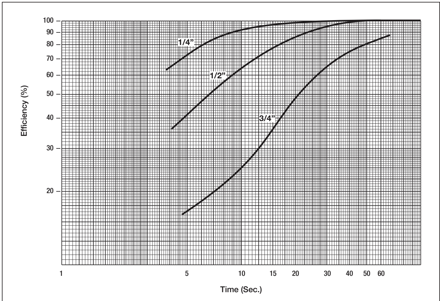
Figure 7: Screenability Characteristic, Frac Sample FS-2
