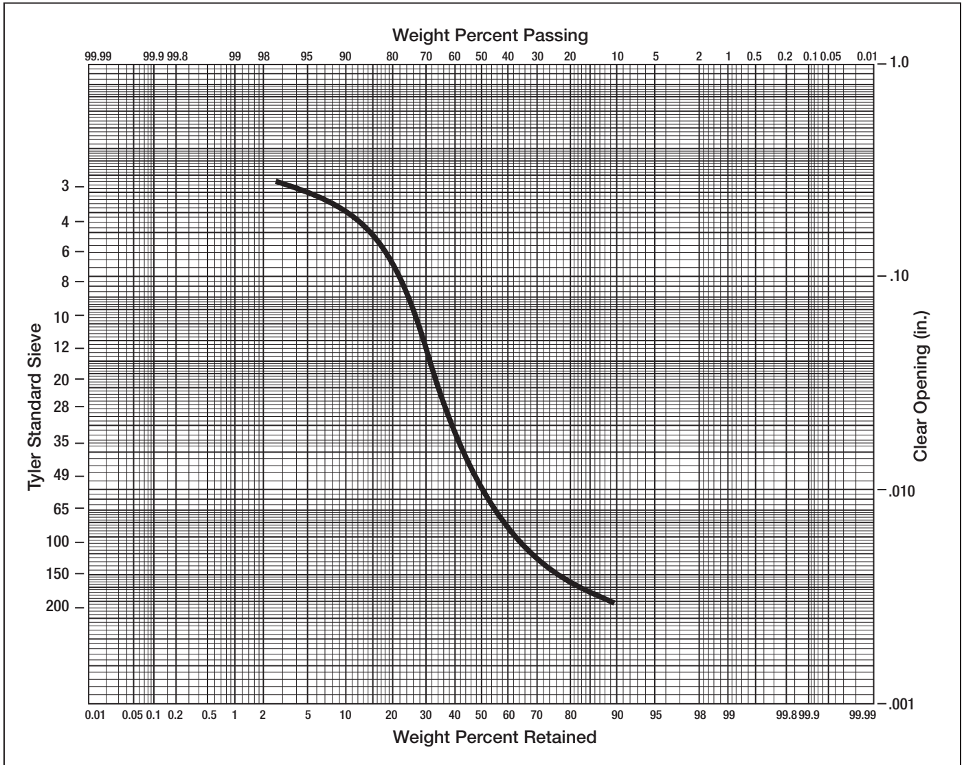
Figure 2: Communitized limestone size distribution
